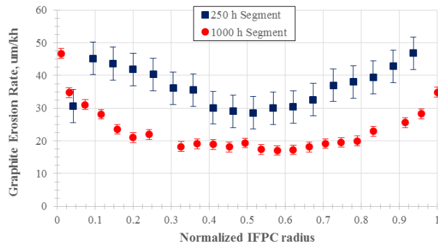
Figure 10. Graphite erosion rates of the TDU-1 IFPC for two segments of the 2016 1700 h wear test. 9
