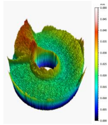
Figure 13. Deposition on the TDU-1 keeper following the two short duration wear tests in VF-6.
