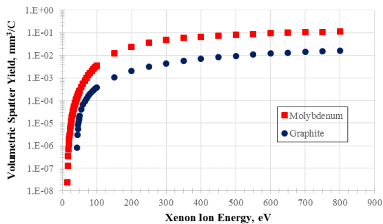
Figure 24. Mo to C volumetric sputter yields as a function of normal-incident Xe II ion energies. 21
