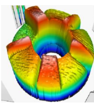
Figure 12. Erosion of the TDU-3 keeper during each of the short duration wear tests in VF-5.
