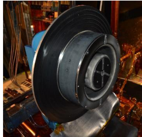
Figure 2. TDU-3 in VF-5 configured for short-duration wear testing.
