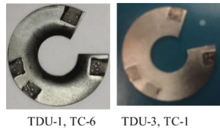
Figure 14. Comparison of Mo keeper masks for TDU-1 and TDU-3 for similar operating conditions.
