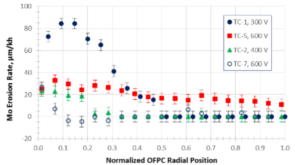
Figure 23. OFPC Mo strip erosion as a function of normalized OFPC radius for several test conditions.
