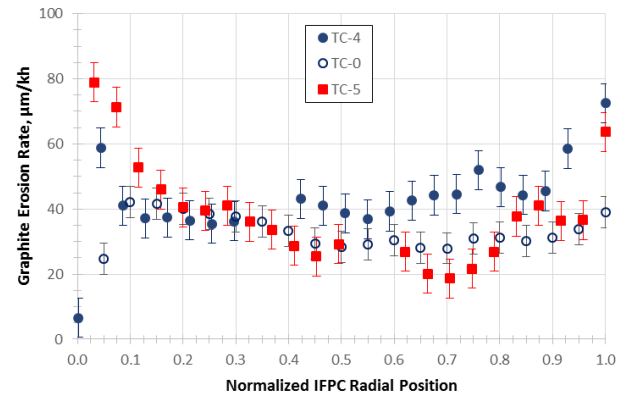
Figure 18. Comparison of IFPC erosion as a function of magnetic field for V_a=600 V in VF-5. Note that TC-5 has a 125% higher B-field.
