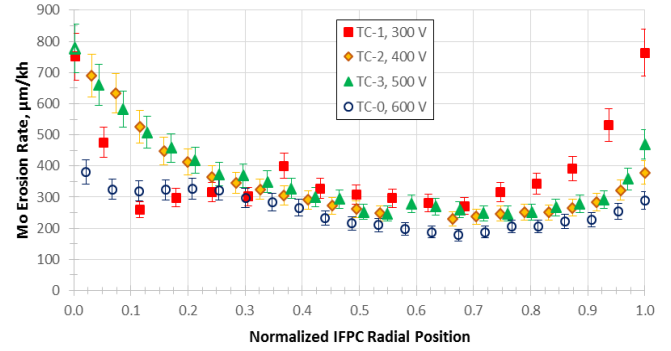
Figure 17. Comparison of Mo strip erosion across the radius of the IFPC.
