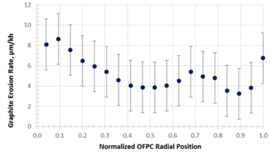
Figure 22. OFPC erosion as a function of normalized OFPC radius.
