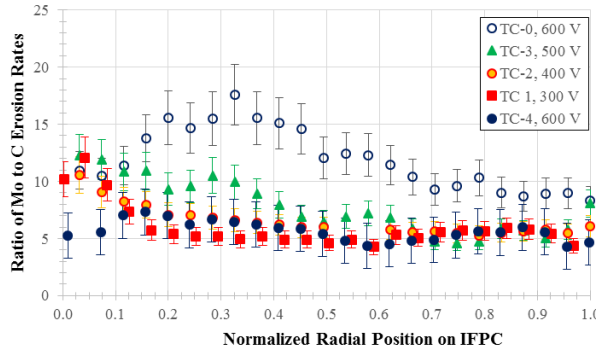
Figure 26. Ratios of Mo to C IFPC erosion rates as a function of discharge voltage.
