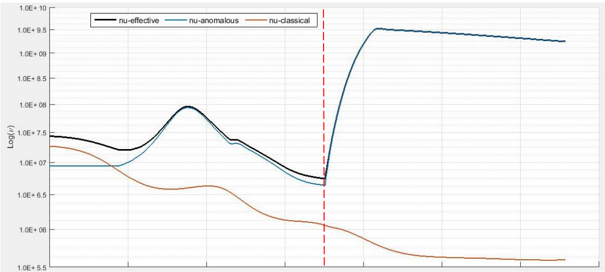
Figure 2. Final profiles of effective, anomalous and electron-neutral collision frequencies from the “Complemented Code”
