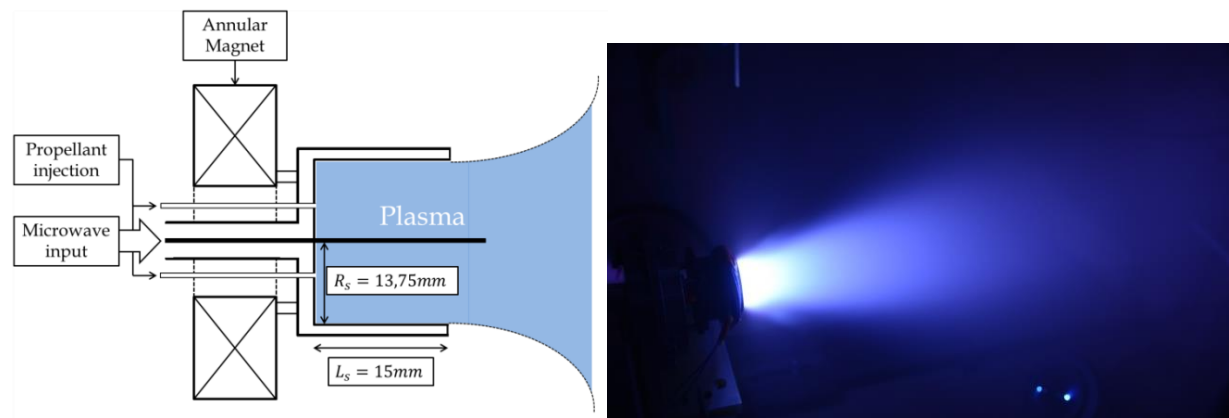
Figure 1. Schematic of the permanent magnet ECR plasma thruster and image of the thruster operated with xenon.
