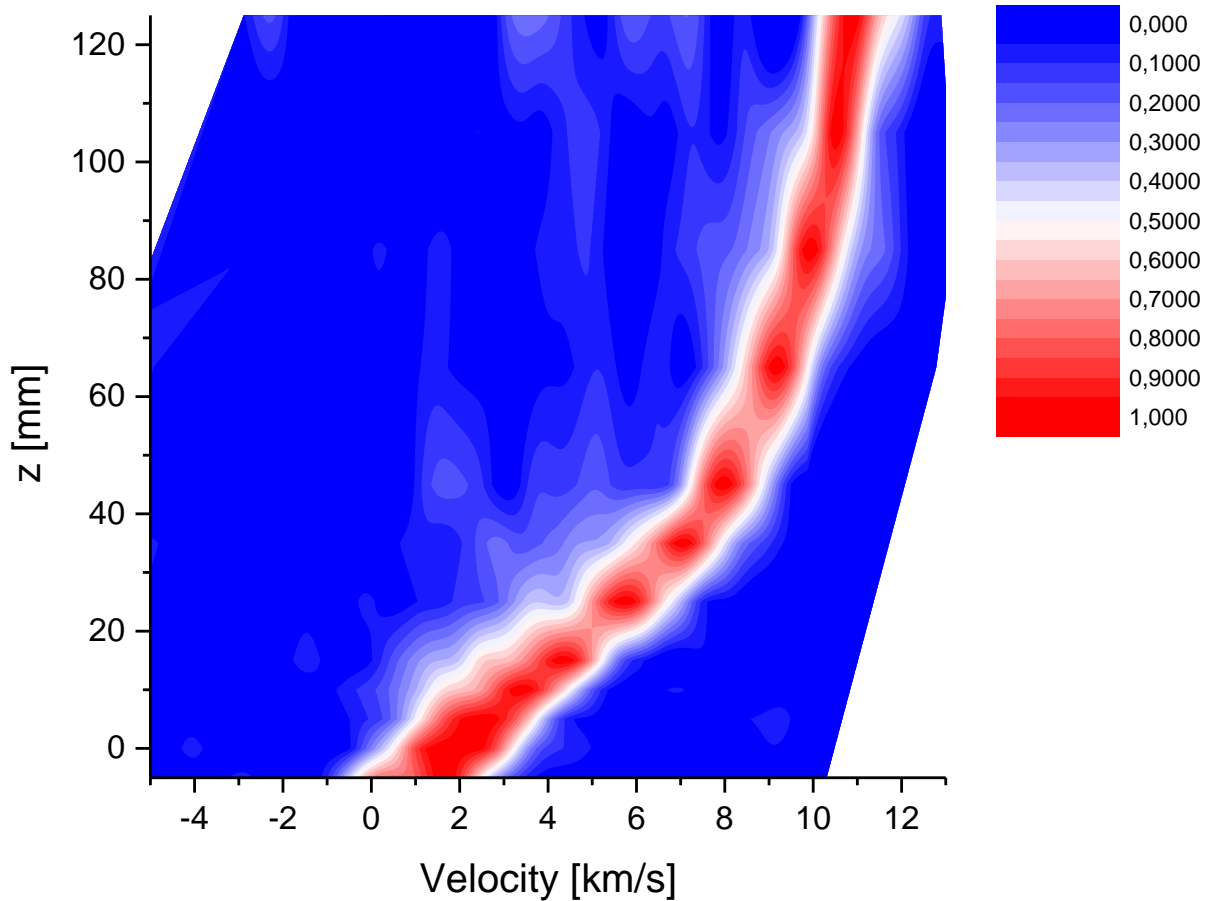
Figure 7. 2D mapping of the IVDF of \text{Xe}^+ in the magnetic nozzle. Xenon flowrate: 2 sccm.
