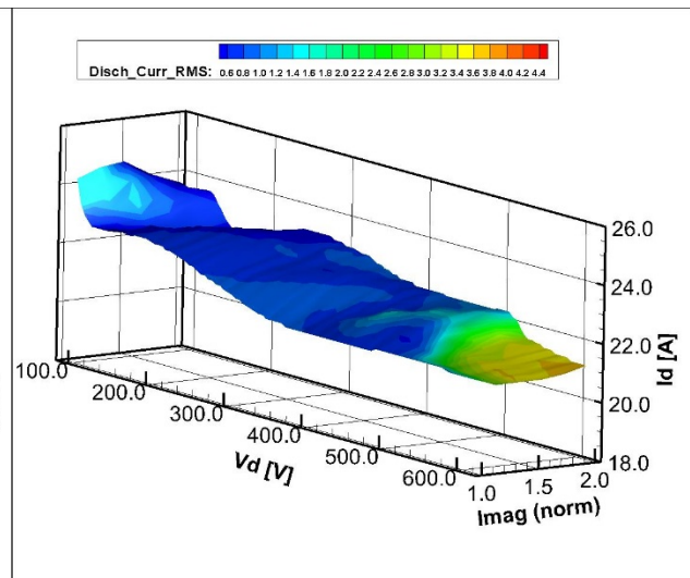
Figure 50. TDU-3 IVB map of discharge current RMS at 20.6mg/s at a CFF of 5% for discharge voltages of 100V to 610V and normalized magnetic field strength of 1 to 2.
