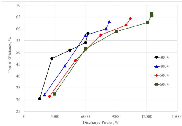
Figure 5. TDU-3 thrust efficiency variation for discharge voltage operation of 300V, 400V, 500V, and 600V.
