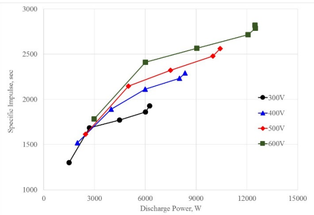
Figure 6. TDU-3 specific impulse variation for discharge voltage operation of 300V, 400V, 500V, and 600V.
