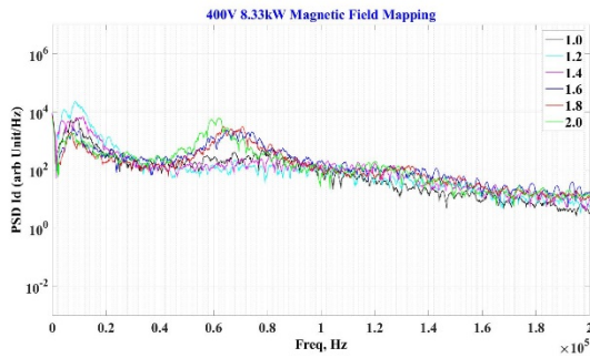
Figure 24. TDU-3 PSD profiles for thruster operation at 400V/8.33kW as a function of the normalized magnetic field.
