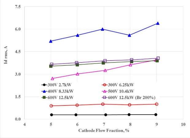
Figure 28. TDU-3 discharge current RMS profiles for thruster operation at RFCs as a function of the CFF.
