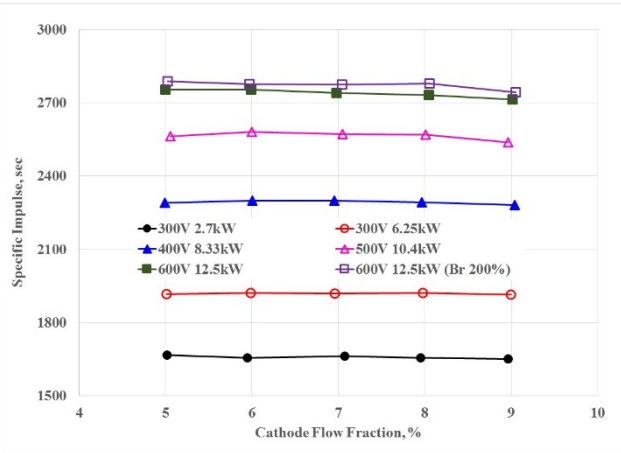
Figure 11. TDU-3 specific impulse magnitudes for thruster operation at the RFCs as a function of the cathode flow fraction (CFF).
