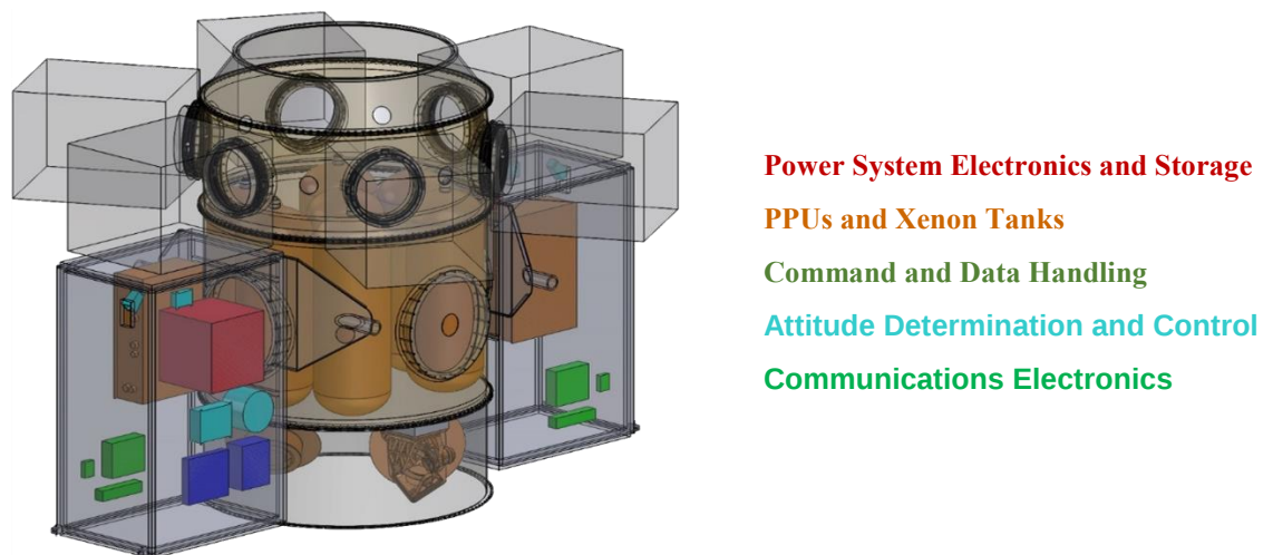
Figure 16. SEP-ESPA Case 1 Transparent View (with subsystem elements identified)
