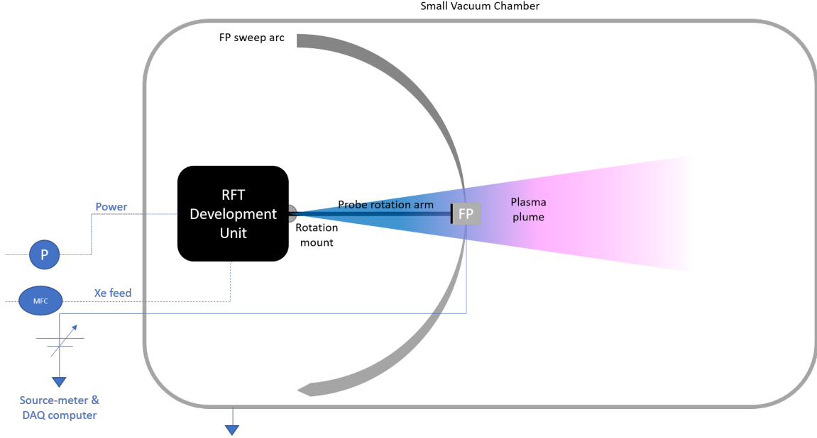
Figure 9: A representative diagram of the test setup at Phase Four for probe testing in the RFT plume. The Faraday probe (FP) is shown on a rotational mount, colocated with the RFT thruster orifice. Power and mass flow control are represented by the ‘P’ and ‘MFC’ blocks in the diagram.
