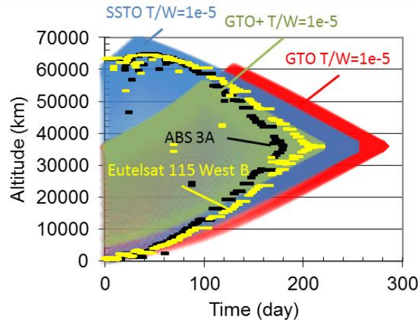
Figure 8. Spacecraft altitude during transfer to GEO assuming several EOR mission scenarios compared to actual Eutelsat 115 West B and ABS 3A trajectories
