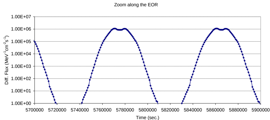
Figure 6. Evolution of electron flux at 2 MeV on a part along the EOR for the SSTO mission
