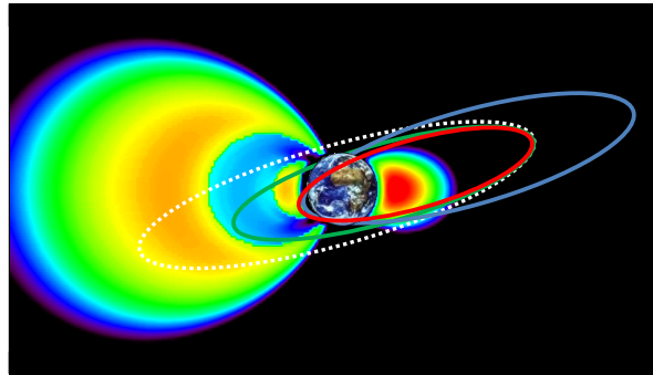
Figure 1. Schematics of orbital injections of GEO satellites (red: GTO, green: GTO+, blue: SSTO) plotted with fluxes of high energy electron (left part) and proton (right part) trapped in the radiation belts
