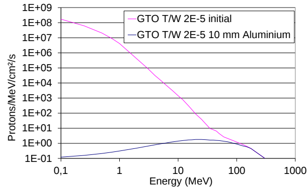
Figure 13. Average proton flux along the EOR GTO T/W = 2 \times 10^{-5} scenario (in pink) and corresponding flux across 10 mm thick aluminum (in blue)
