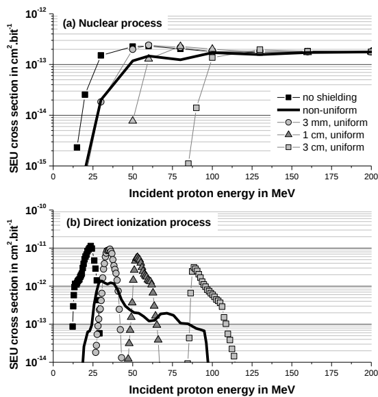
Figure 16. (a) Nuclear and (b) direct ionizing proton SEU cross section of a 28-nm FDSOI technology considering several shielding conditions ( \emptyset , 3 mm, 1 cm, 3 cm uniform shielding and no uniform shielding).
