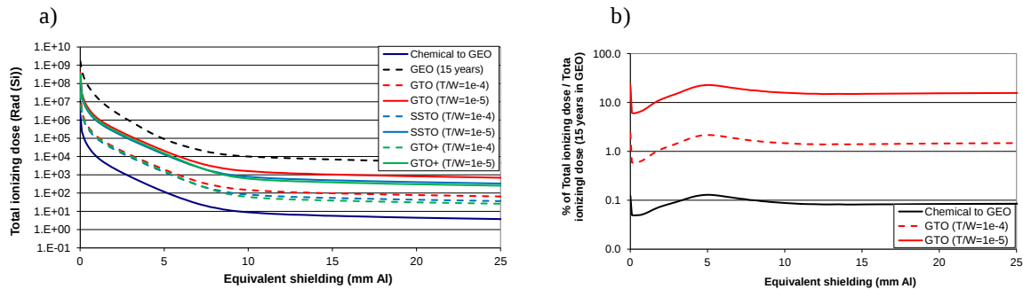
Figure 12. (a) Total ionizing dose received during transfers to GEO compared with the total ionizing dose received during 15 years at GEO and (b) Total dose received during the transfer to GEO by chemical propulsion and by two electrical propulsion scenarios, in % of the dose received during the 15 years mission at GEO
