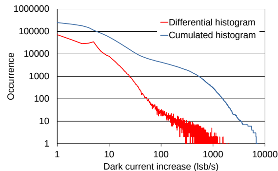
Figure 15. Differential and cumulative histograms (with a bin of 1 lsb/s) of the dark current increase at 300 K and after proton irradiation representative of a 140 days EOR GTO mission.
