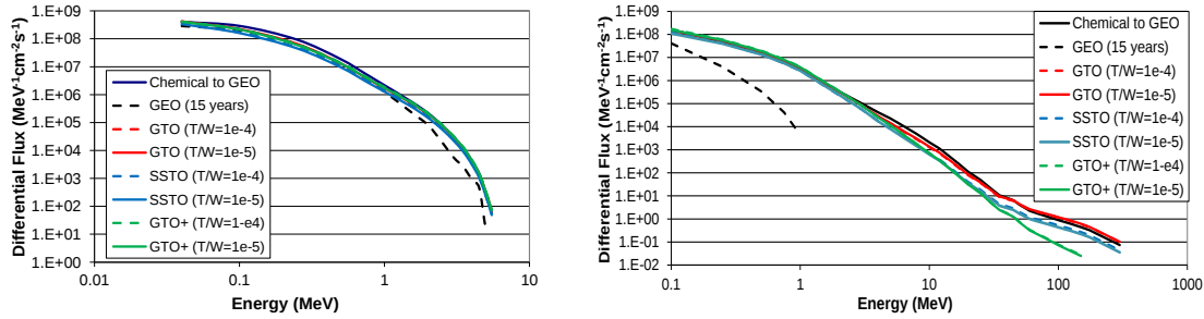
Figure 9. Electron (left) and proton (right) average differential fluxes of, assuming several scenarios for transfer to GEO, compared to the 15 years mission at GEO alone.
