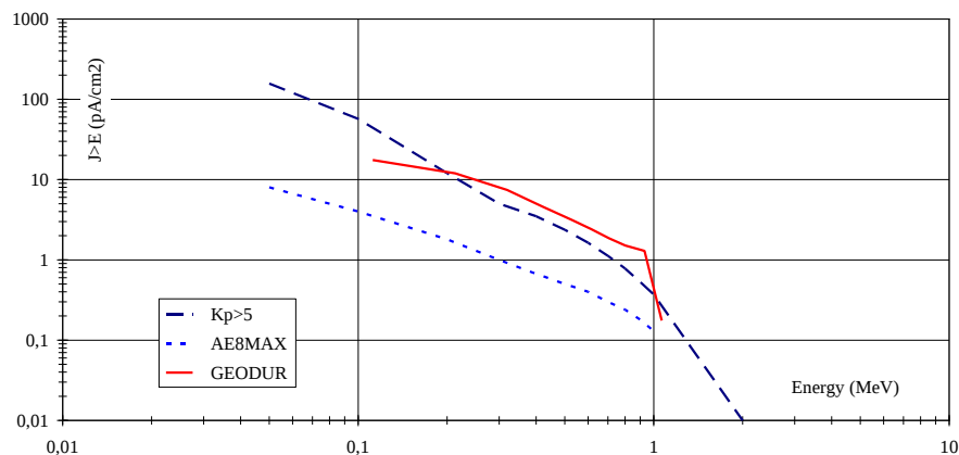
Figure 4. GEODUR electron spectrum compared to GEO AE8 max and Kp>5 spectra
