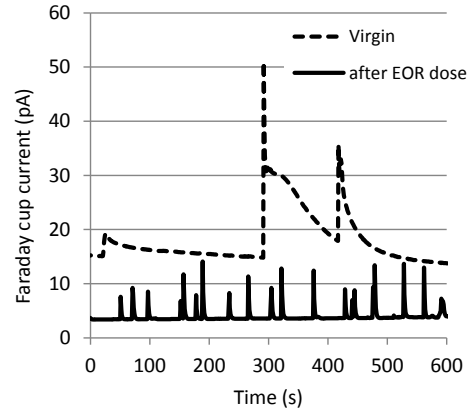
Figure 19. Time evolution of the electron current collected by faraday cups during ESD test protocol. The dashed and the plain lines have been obtained during step 2 and step 7, respectively; both at V_{bias} = -800 V.
