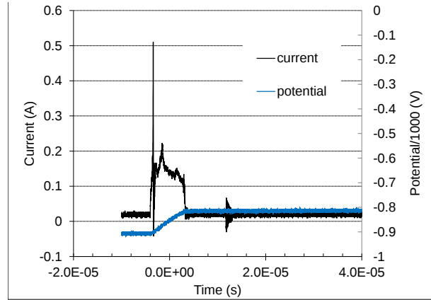
Figure 18. Electrical signal of a typical ESD produced on the test setup of Figure 2
