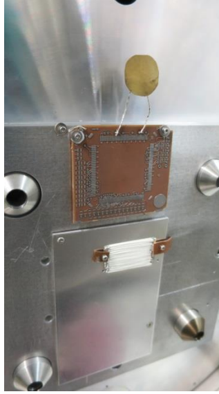
Figure 7. View of the PCB and ETFE wires tested in the GEODUR test facility
