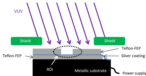
Figure 2. Schematics of the samples used to generate electrostatic discharges.
