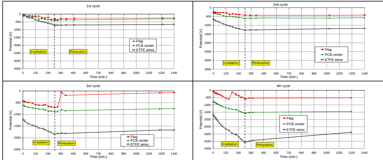
Figure 20. Evolution of surface potential on PCB (flag and center of PCB) and ETFE wires along the 4 irradiation cycles
