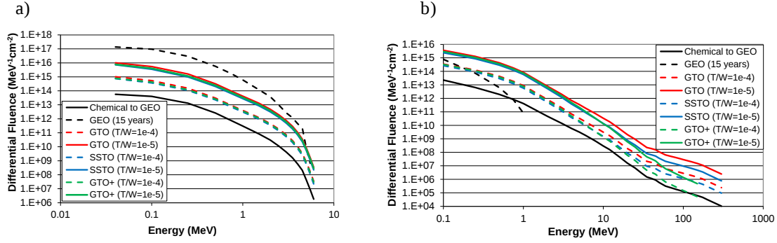
Figure 11. Differential fluence of (a) electrons and (b) protons under the same conditions as in Figure 9.
