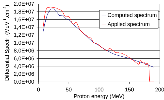
Figure 14. Comparison between the proton fluence representing the GTO EOR mission (referred as computed) and the fluence actually applied during the experimental campaign.
