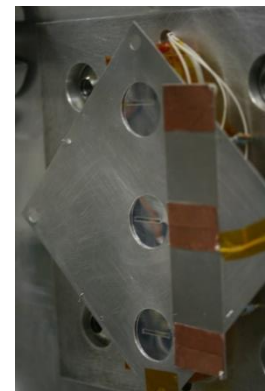
Figure 3. Picture of the three samples located inside the SIRENE facility.
