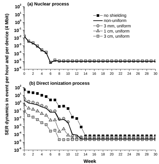
Figure 17. (a) Nuclear and (b) direct ionizing proton SER dynamics of a 28-nm FDSOI technology considering several shielding conditions ( \emptyset , 3 mm, 1 cm, 3 cm uniform shielding and no uniform shielding) and all-electric telecom satellite mission.
