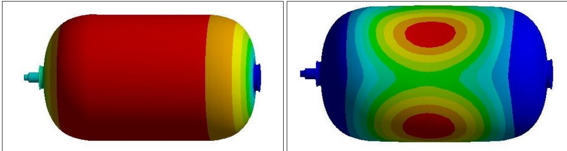
Figure 3. XPT's First Axial and Lateral Modes
