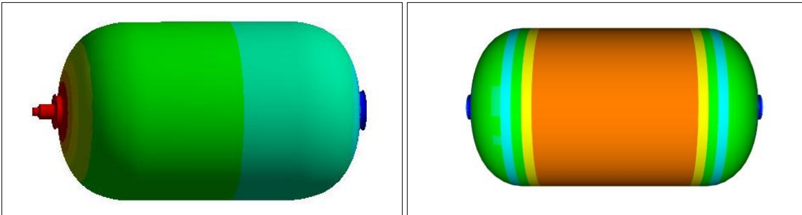
Figure 4. Axial deformation of liner and stress distribution of composite overwrap under MEOP
