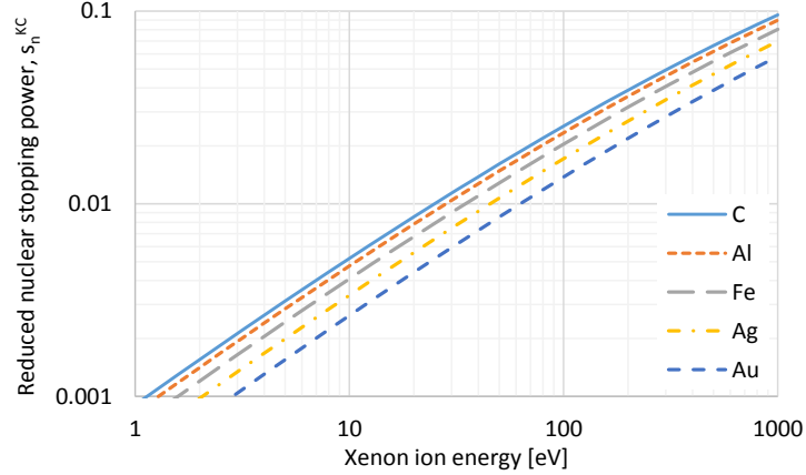
Figure 4: Reduced nuclear stopping power for xenon ion impacts with various elements
