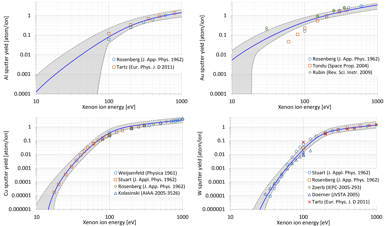
Figure 7: Aluminum (top-left), gold (top-right), copper (bottom-left), and tungsten (bottom-right) sputter yields from low energy xenon ions at normal incidence with measured data compared to 50% likelihood bounds on the yield curves
