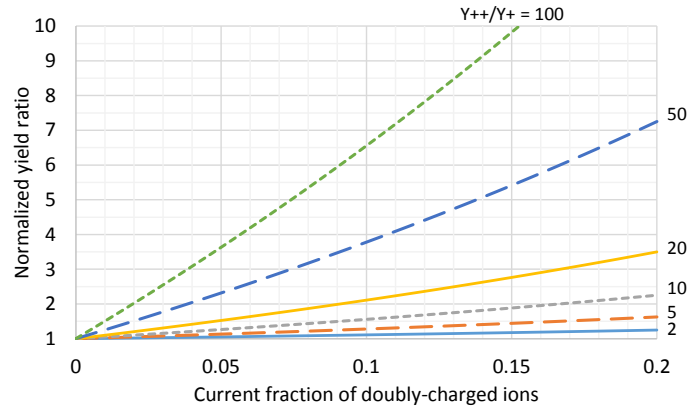
Figure 1: Change in total yield due to double-charged ions
