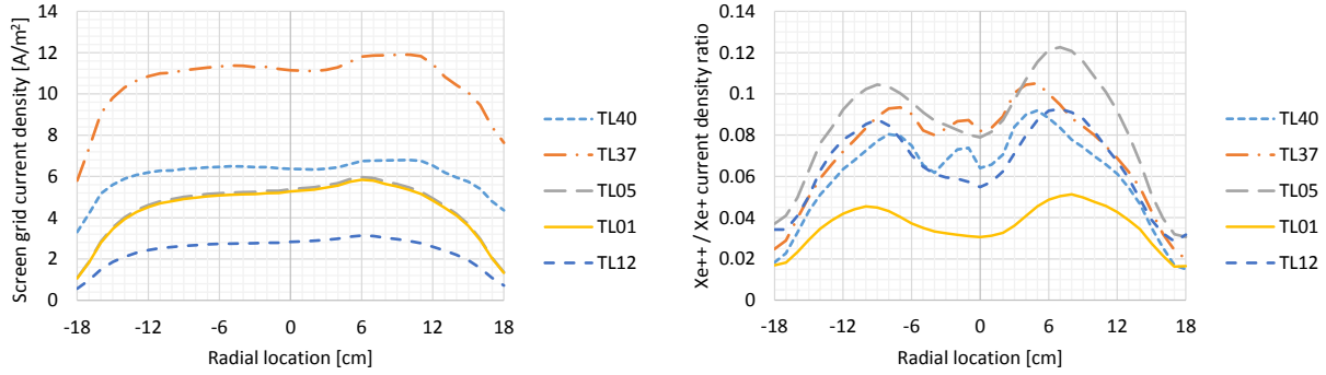
Figure 2: Current density profiles (left) and doubly-to-singly-charged ion ratios (right) at the screen grid
