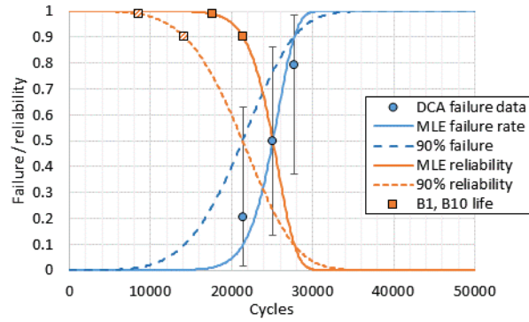
Figure 18: NCA heater failure rate and reliability
