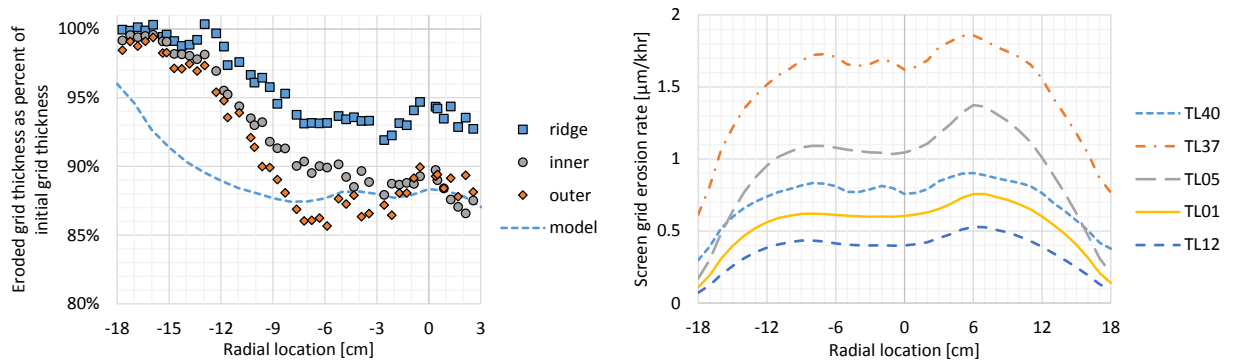
Figure 3: Total screen grid erosion comparison to LDT measured profiles (left) and estimated flight model erosion rates (right)
