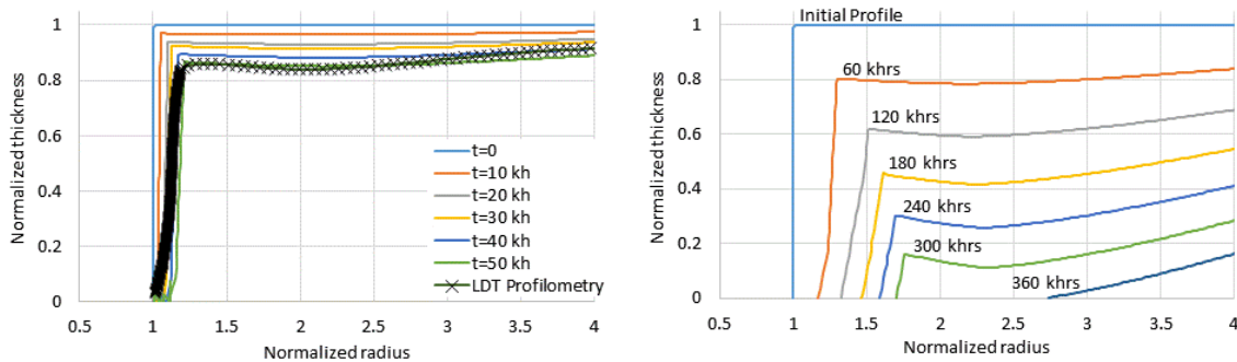
Figure 8: Modeled wear of the graphite DCA keeper for the LDT (left) and eventual failure (right).
