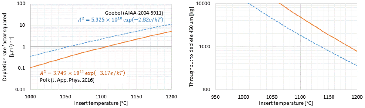
Figure 12: Barium depletion rate factors (left) and throughput (based on TL37 flow rate) to deplete 450 μm of barium (right)
