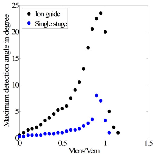
Figure 5. Simulation of Variation of the lens efficiency with V_{lens}/V_{em}
