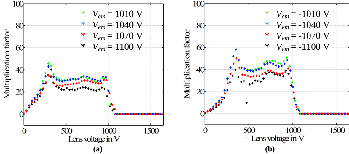
Figure 11. Measured Lens efficiency for different emission voltages in positive (a) and negative (b) polarities respectively from microfabricated electrospray device with 300 \mu\text{m} extractor diameter.
