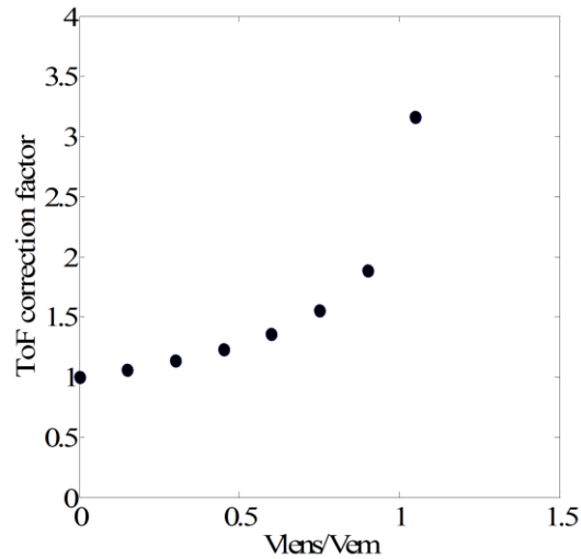
Figure 6. Simulation of variation of the ToF correction
