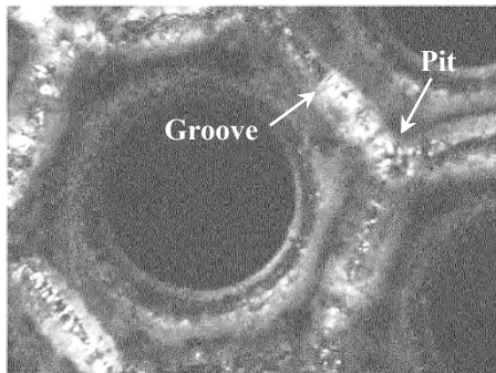
Figure 1. The NEXT LDT accelerator grid center aperture at 19,520 h showing the pit and groove erosion pattern. Darker regions are net carbon deposition while lighter regions are net molybdenum erosion.
