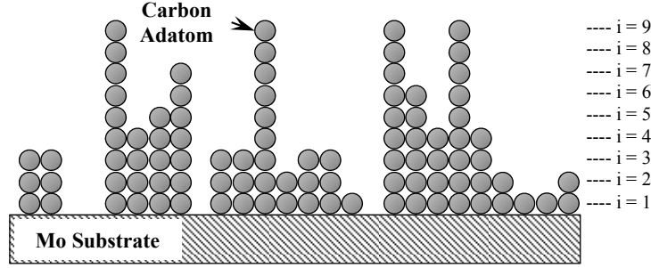
Figure 4. Illustration of the surface coverage model developed for this study.
