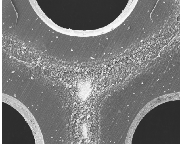
Figure 3. Scanning electron photomicrograph of the downstream NSTAR accelerator grid at 11.8 cm from the center of the grid. 12 White areas are molybdenum and gray areas are carbon.
