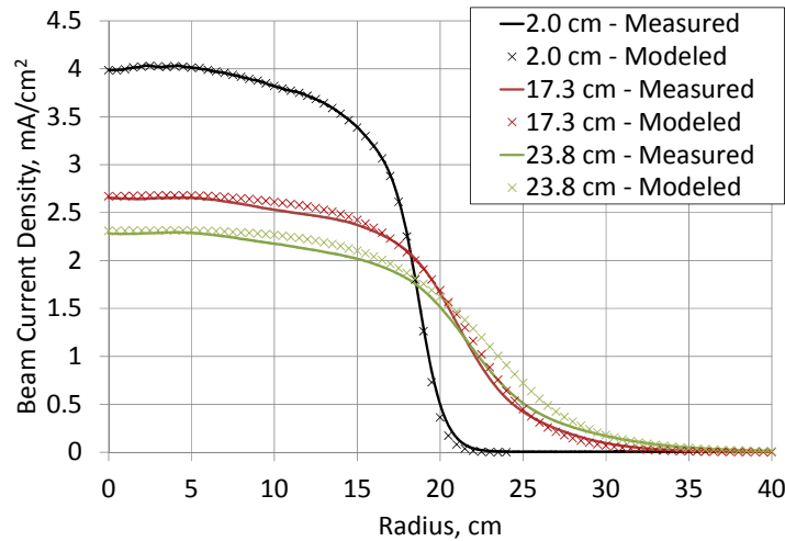
Figure 6. Measured and predicted beam current densities for the NEXT LDT thruster at full power at various axial locations.
