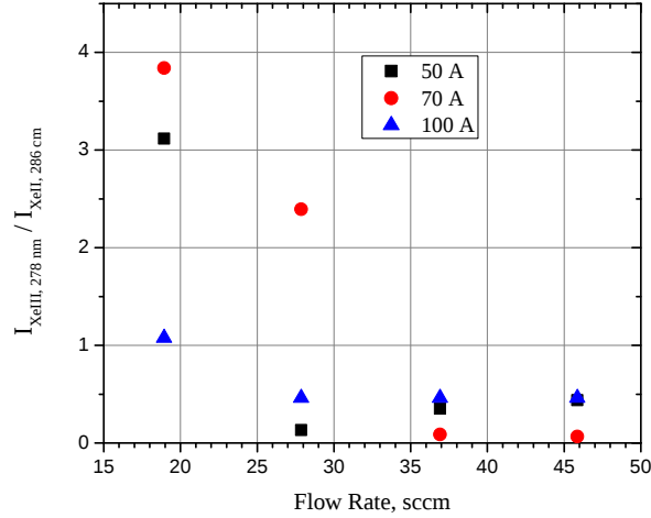
Figure 11: I_{\text{Xe III}, 278 \text{ nm}} to I_{\text{Xe II}, 286 \text{ nm}} as a function of mass flow rate. The ratio provides an indication of the relative concentrations of Xe III and Xe II since T_e \approx \text{constant} .
