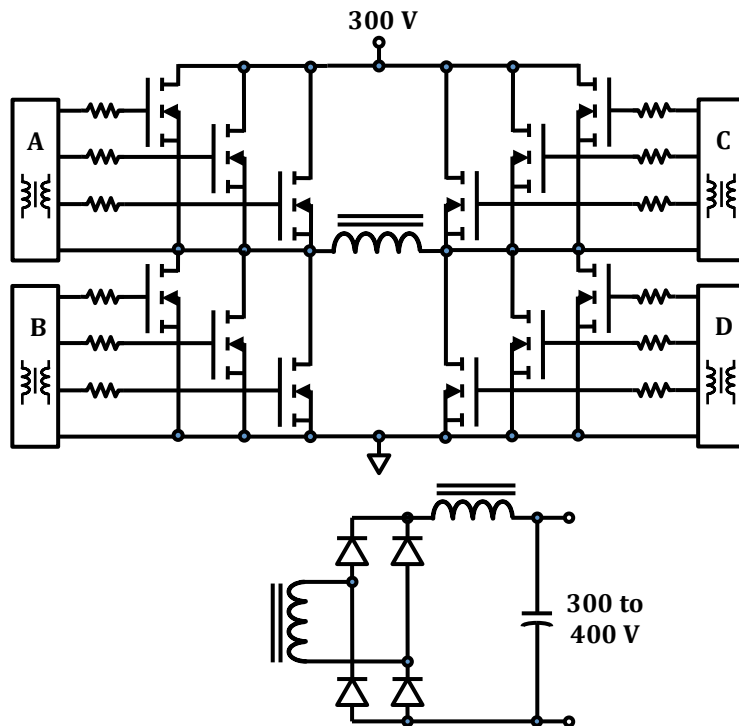
Figure 2, Discharge module simplified schematic
