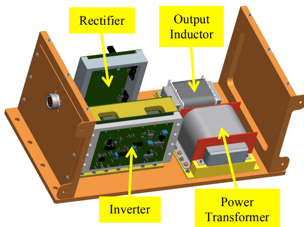
Figure 9, Brassboard discharge module
