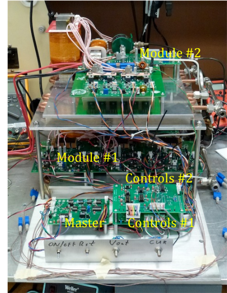
Figure 3, Breadboard discharge power supply
