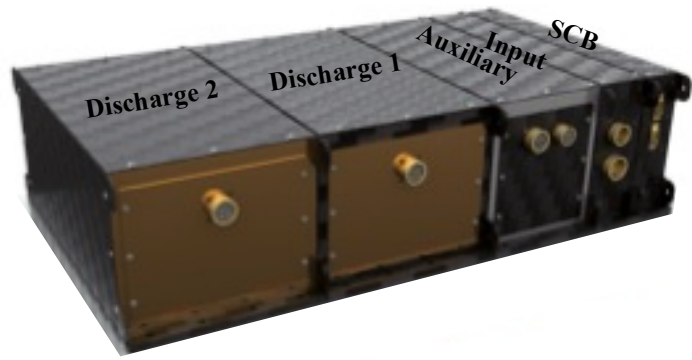
Figure 8, Brassboard PPU
