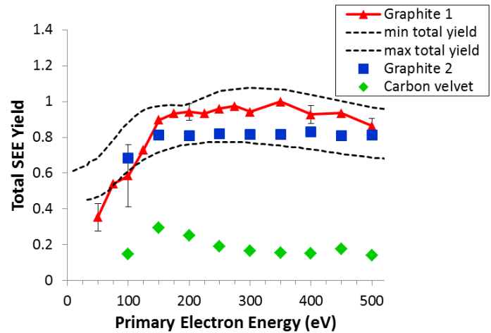
Figure 1. A comparison of the total secondary electron emission yield from graphite and carbon velvet materials. Graphite 1 and Graphite 2 are samples made from the same Poco graphite material. The results for Graphite 1 were obtained using a new PPPL setup for measurements of SEE based on Auger electron spectroscopy [5]. The dashed lines show the range of values for SEE yield from graphite deduced from data available in the literature [5]. SEE yield from Graphite 2 and carbon velvet was measured using the setup described in Ref. [3].
