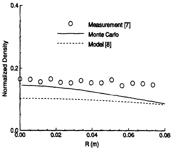
Figure 4: Radial variation in normalized xenon density at a distance of 15 cm from the thruster exit plane.
