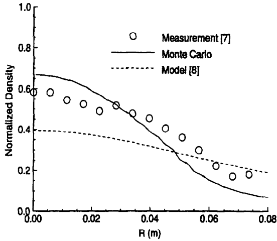
Figure 3: Radial variation in normalized xenon density at a distance of 4.5 cm from the thruster exit plane.
