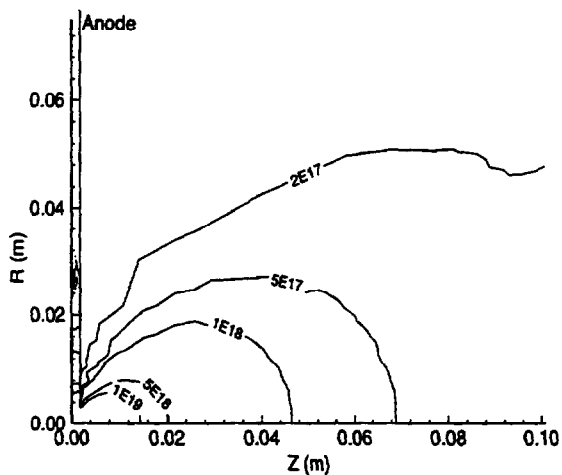
Figure 8: Contours of number density for the plasma contactor plume.
