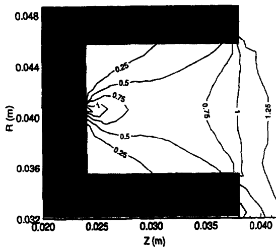
Figure 12: Computed Mach number contours of neutral flow inside the Stanford Hall thruster.
