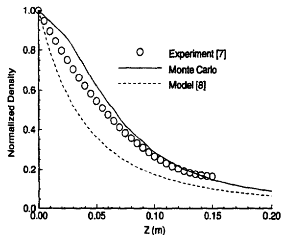
Figure 2: Variation in normalized xenon density along the thruster plume axis.
