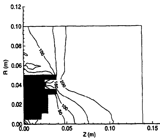
Figure 14: Computed velocity contours of neutral flow in the plume of the Stanford Hall thruster.
