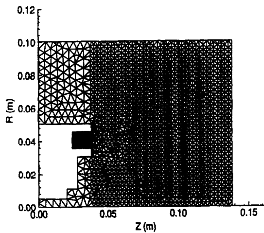
Figure 11: Unstructured grid employed for simulation of neutral flow through the Stanford Hall thruster.
