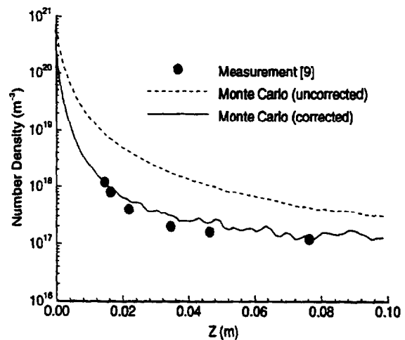
Figure 10: Density along the axis of the plasma contactor plume.
