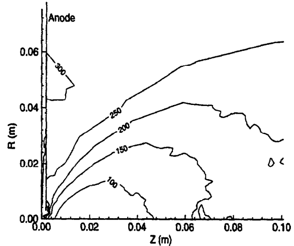
Figure 9: Contours of translational temperature for the plasma contactor plume.
