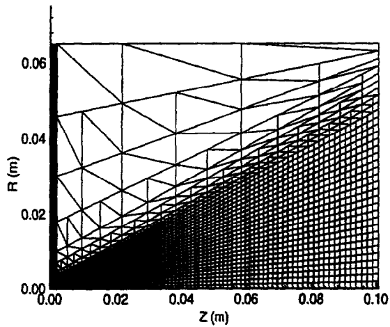
Figure 7: Grid employed for Monte Carlo computation of plasma contactor plume illustrating mixture of quadrilateral and triangular cells.
