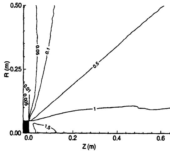
Figure 5: Ratio of number densities: Monte Carlo prediction divided by analytical model.
