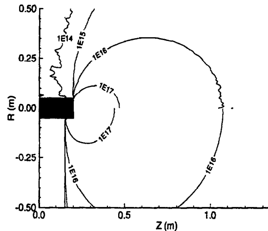
Figure 1: Contours of number density in \text{m}^{-3} for the plume of the UK-10 ion thruster: Monte Carlo (upper) and analytical model (lower).
