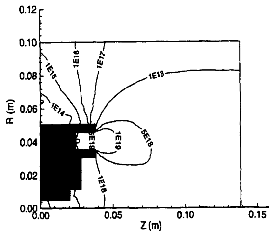
Figure 13: Computed number density contours of neutral flow in the plume of the Stanford Hall thruster.
