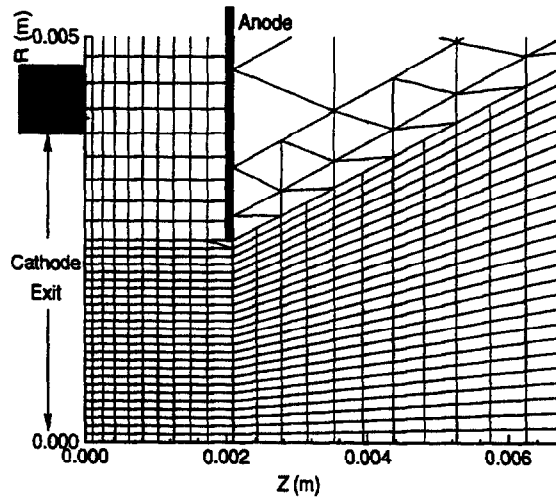
Figure 6: Close-up view of computational grid showing geometry of cathode and anode for plasma contactor.
