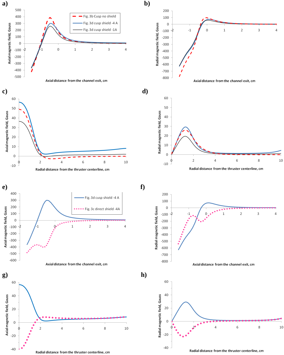
Figure 5. Simulation results of the axial and radial profiles of the magnetic field for the 2.6 cm channel diameter CHTem thruster. The axial profiles along the channel are shown for R = 1 cm from the thruster centerline. The radial profiles are shown at Z = 1 cm from the channel exit. Figures a-d compare the cusp configuration of the CHTem without shield (Fig. 3b) with the shielded configuration of the cusp CHTem (Fig. 3d) at two different shield coil currents: -1 A and -4 A. Figures e-h compares the axial and radial profiles of the magnetic field for two magnetically shielded configurations: direct (Fig. 3c) and cusp (Fig. 3d) at the same shield coil current of -4 A.
