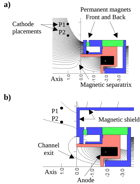
Figure 2. Magnetic field (simulations) for the the 2.6 cm diameter CHT with with permanent magnets a) without the magnetic shield, 3 B_{zmax} = 2.5 kGauss at the magnetic mirror and (b) with the magnetic shield, 8 B_{zmax} = 1.76 kGauss. All dimensions are in cm. Magnetic iron parts made from low carbon steel are marked in blue. Samarium-cobalt permanent magnets are marked in green. Two cathode placements, P1 and P2 used in CHTpm experiments are also shown.
