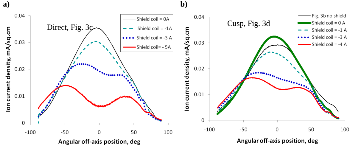
Figure 7. Angular ion current density distribution measured for the shielded CHT thruster with electromagnet coils under variations of the shield coil current: a) direct configuration shown in Fig. 3c and b) cusp configuration shown in Fig. 3d. In addition, the results for the cusp configuration of the CHTem without the magnetic shield and the shield coil (Fig. 3b) are shown on the right figure. Fig. 5 compares the magnetic field distribution for some of these thruster configurations. Measurements were conducted for the discharge voltage of 250V, Xenon gas, anode gas flow rate of 3.5 sccm and the cathode gas flow rate of the 2 sccm. For all magnetically shielded CHTem configurations, the cathode was placed at the distance of 1 cm from the channel exit in the axial direction and about 6 cm from the thruster centerline in the radial direction.
