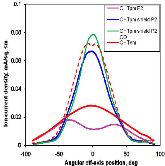
Figure 6. Effect of the magnetic shield on the plasma plume of the CHTpm thruster. The results of the plume measurements for the CHTpm and CHTem thrusters with the auxiliary keeper discharge (so-called current overrun (CO) regime with the keeper current of 2.5 A) are also shown. All thrusters were operated at the discharge voltage of 250 V and Xenon gas flow rate of 3.5 sccm. For the CHTpm thrusters, the cathode placement P2 is shown in Fig. 2. 11 For the CHTem thruster, the cathode placement was different: the cathode outlet orifice was located approximately 5.4 cm away radially and 2 cm downstream from the center of the channel exit.
