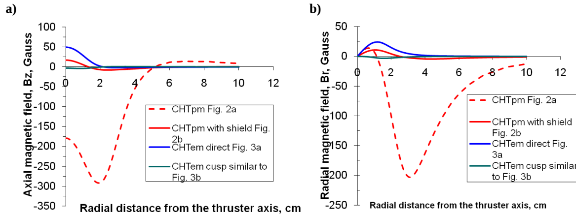
Figure 4. Simulation results of the magnetic field distribution (for the axial (a) and radial (b) components of the magnetic field) in the radial direction at 1 cm from the exit of the 2.6 cm diameter channel of the cylindrical thruster configurations shown in Figs. 2 and 3: CHTpm with and without magnetic shield and CHT with electromagnet coils without the magnetic shield. For the cusp configuration of the CHTem, the front coil current is -2 A and the back coil current is +2.5 A.
