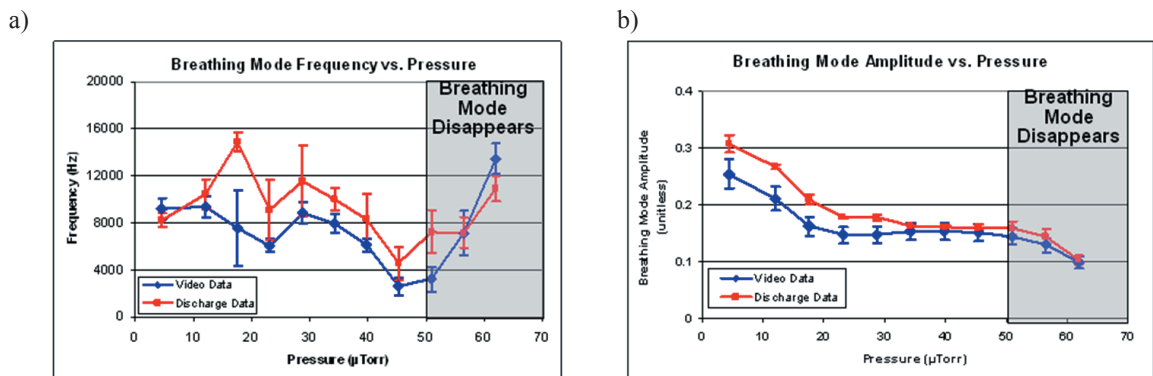
Figure 6. Variations of the frequency (a) and COV (b) of the breathing oscillations with the background pressure.
