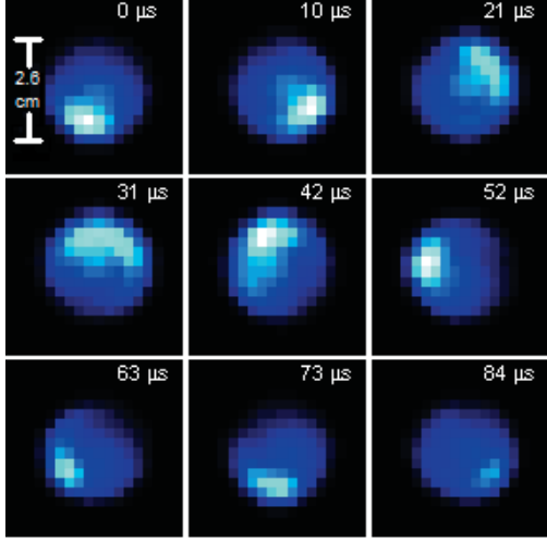
Figure 2. Sequence of camera images show counter-clockwise rotation, in the ExB direction, in the cusp configuration of the 2.6 cm CHT thruster. This spoke was not observed for the direct magnetic configuration of the CHT. 4
