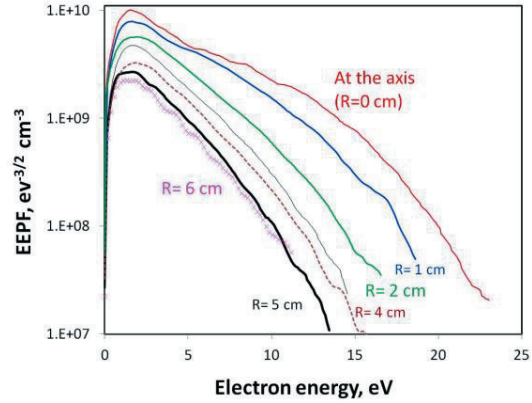
Figure 5. Penning discharge measurements with VGPS probe - spatial variations of the electron energy probability function (EEDF) at the magnetic field of 35 Gauss. Hot electrons near the axis, R \leq 2 cm, could be due to plasma- beam interaction (electron beam from the cathode).
