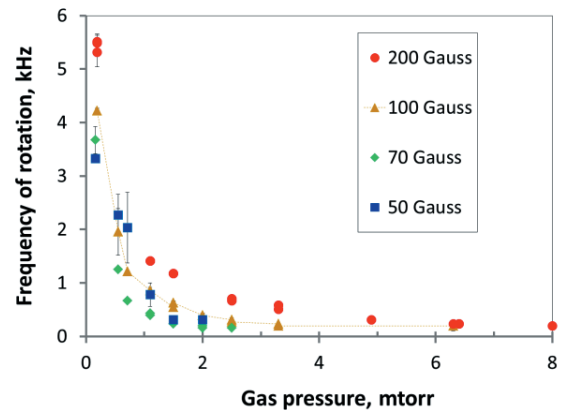
Figure 8. Penning discharge system: The frequency of the rotating spoke oscillations with the background pressure. 13
