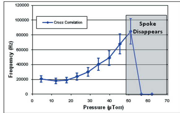
Figure 7. Variations of the frequency of the rotating spoke oscillations with the background pressure. 13
