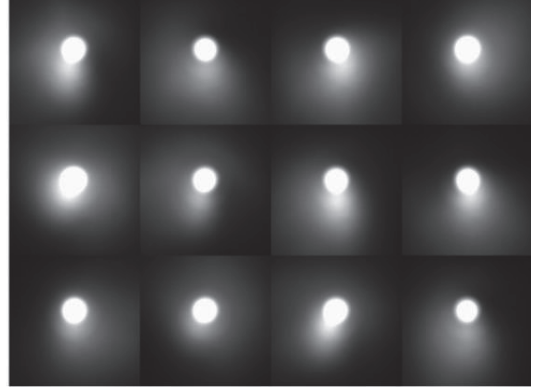
Figure 4. Rotating spoke observed in the Penning discharge at the discharge voltage between the cathode and the chamber of 100 V and the magnetic field of 100 Gauss. Background (xenon) gas pressure is 0.3 mtorr. 2
