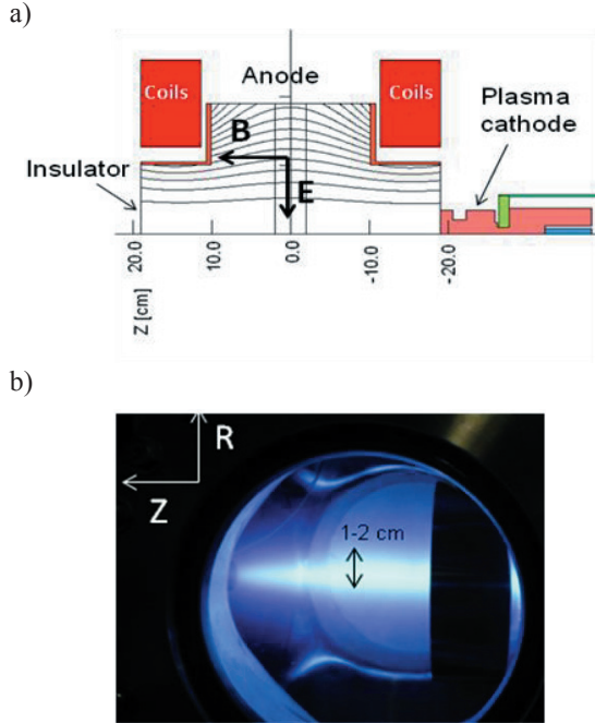
Figure 3. (a) ExB configuration of the Penning DC-RF discharge; b) Xenon operation of the Penning discharge. 2
