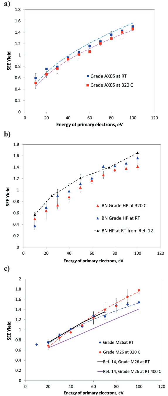
Figure 4. SEE yield for BN grades at room temperature and 320 C: a) Grade AX05; b) Grade HP, and c) Grade M26. In addition, data from other SEE measurements for BN HP (Ref. 12) and M26 (Ref. 14) are shown on Figure b and c, respectively. Dashed lines on figures a) and c) are for Fit 1 and Fit 2 (see Table 1), respectively. Blue and red dashed curves are for room temperature and 320 C respectively
