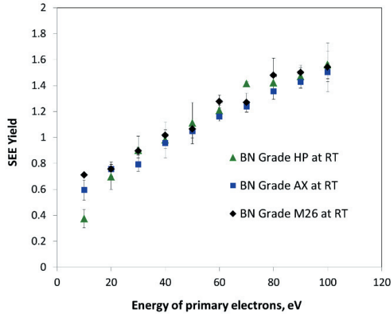
Figure 3. SEE yield for boron nitride grades HP, AX05 and M26 at room temperature.
