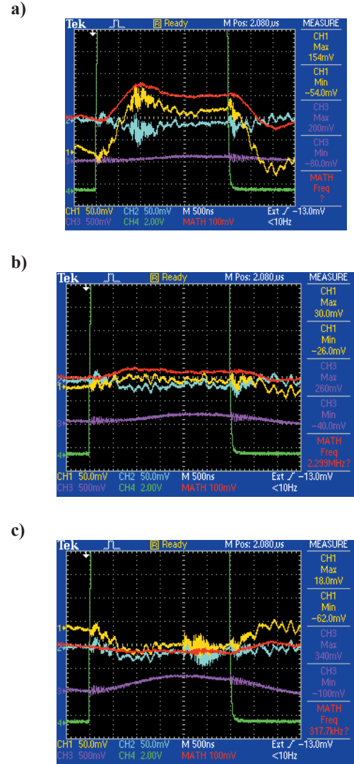
Figure 2. SEE measurements for a BN sample: sample current signal (yellow), Faraday cup (references) signal (magenta), and the processed waveform (red) at beam energy of a) 20eV, b) 50 eV and c) 70 eV. The SEE yield estimated using the sample method (Eq. 1); a) less than 1, b) about 1; and c) more than 1.
