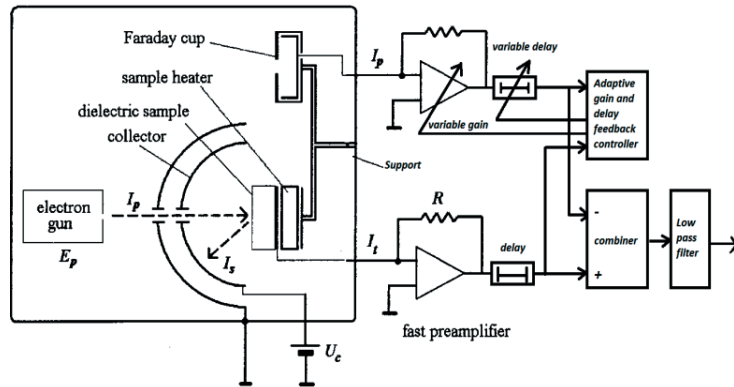
Figure 1. Upgraded setup for low noise and high resolution measurements of the SEE yield from the dielectric materials.
